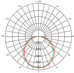
LS-5EHB100W-50K
