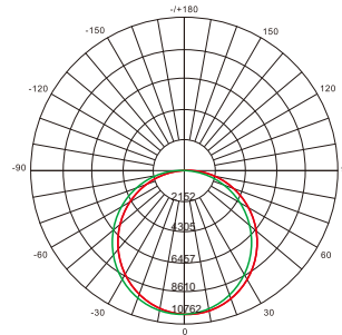
LS-5EHB150WHV-50K
