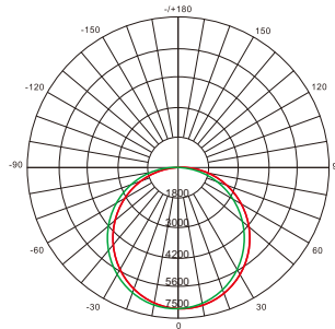
LS-5EHB100WHV-50K
